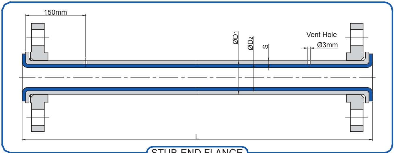
STUB-END FLANGE
