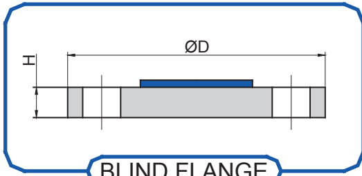
BLIND FLANGE
