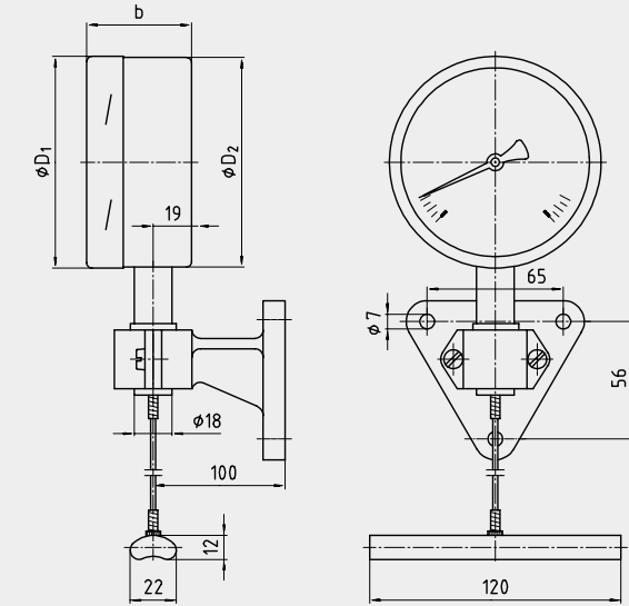
Model F73.XXX, with surface-mounted contact bulb, capillary and surface mounting bracket
