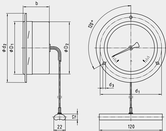
Model F73.XXX, with surface-mounted contact bulb, capillary and 3-hole panel mounting flange
