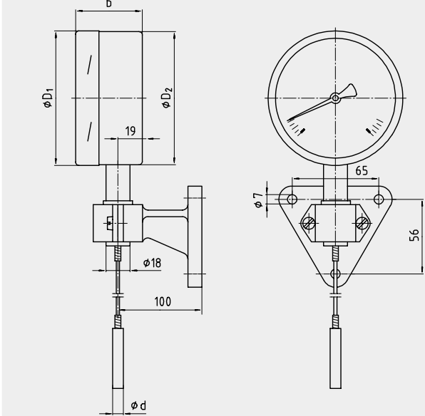
Model F73.XXX, with capillary and surface mounting bracket
