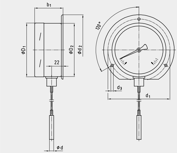
Model F73.XXX, with capillary and 3-hole surface mounting flange
