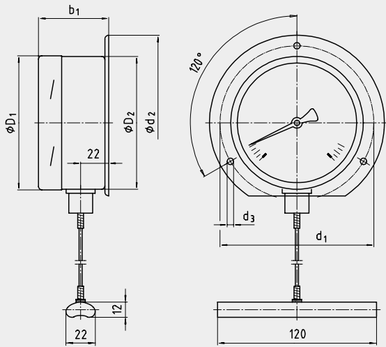
Model F73.XXX, with surface-mounted contact bulb, capillary and 3-hole surface mounting flange
