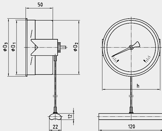
Model F73.XXX, with surface-mounted contact bulb, capillary and triangular bezel with bracket 1)
