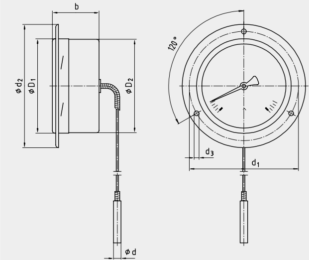
Model F73.XXX, with capillary and 3-hole panel mounting flange
