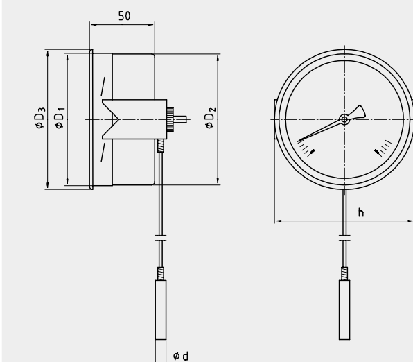
Model F73.XXX, with capillary and triangular bezel with bracket 1)
